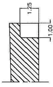
SECTION A-A (FEMALE END) SCALE 1=2
